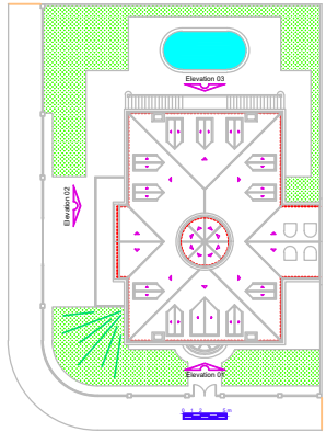
Roof Plan
