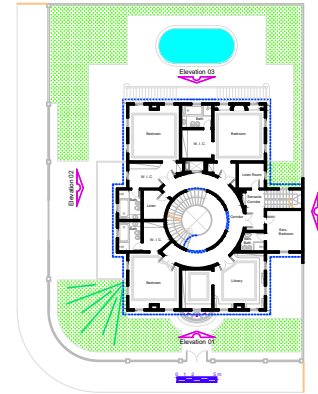
Second Floor Plan A = 295,18 m 2
